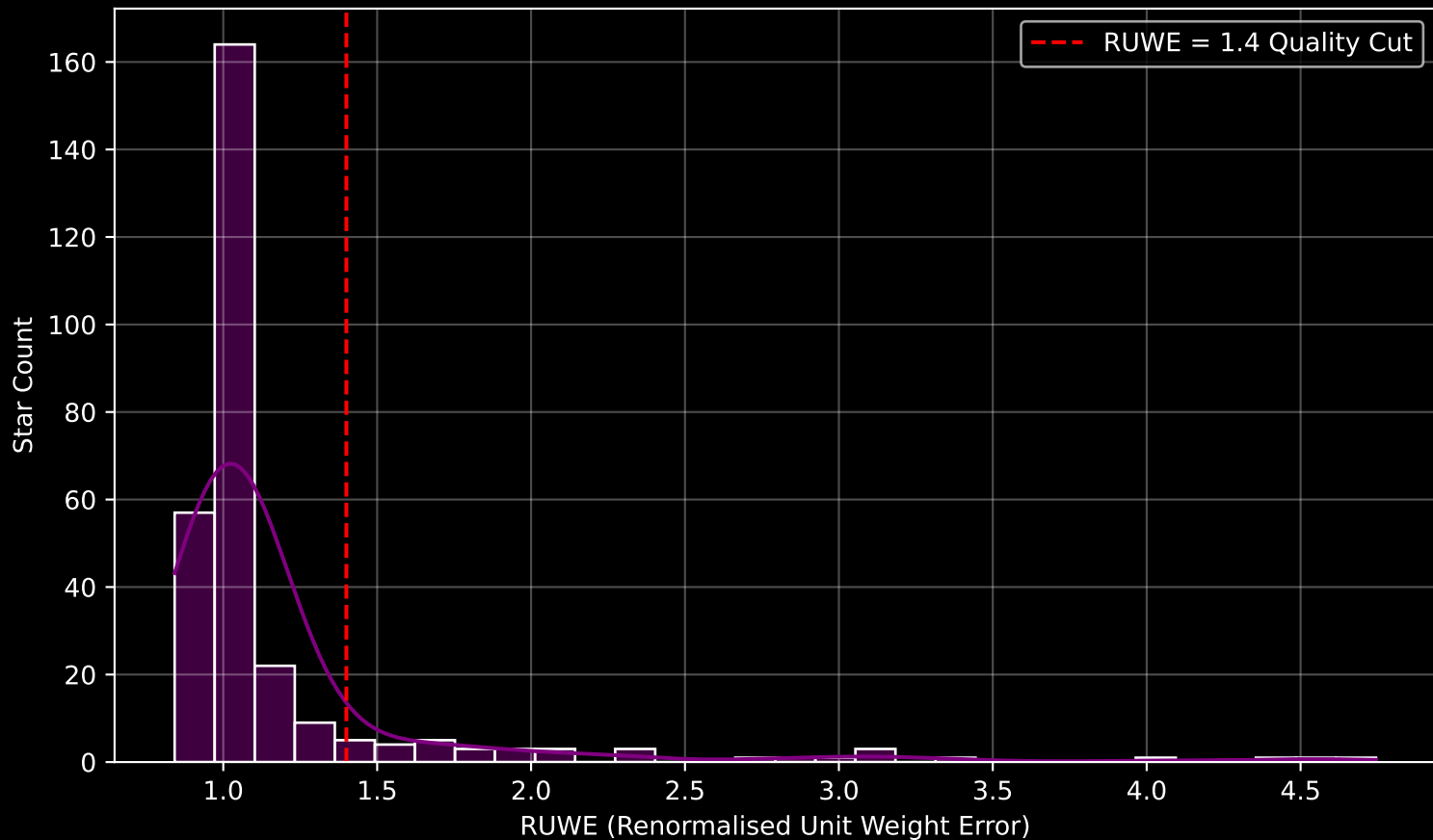
GALAH DR4 Field [397] RUWE Distribution (n= 289)
