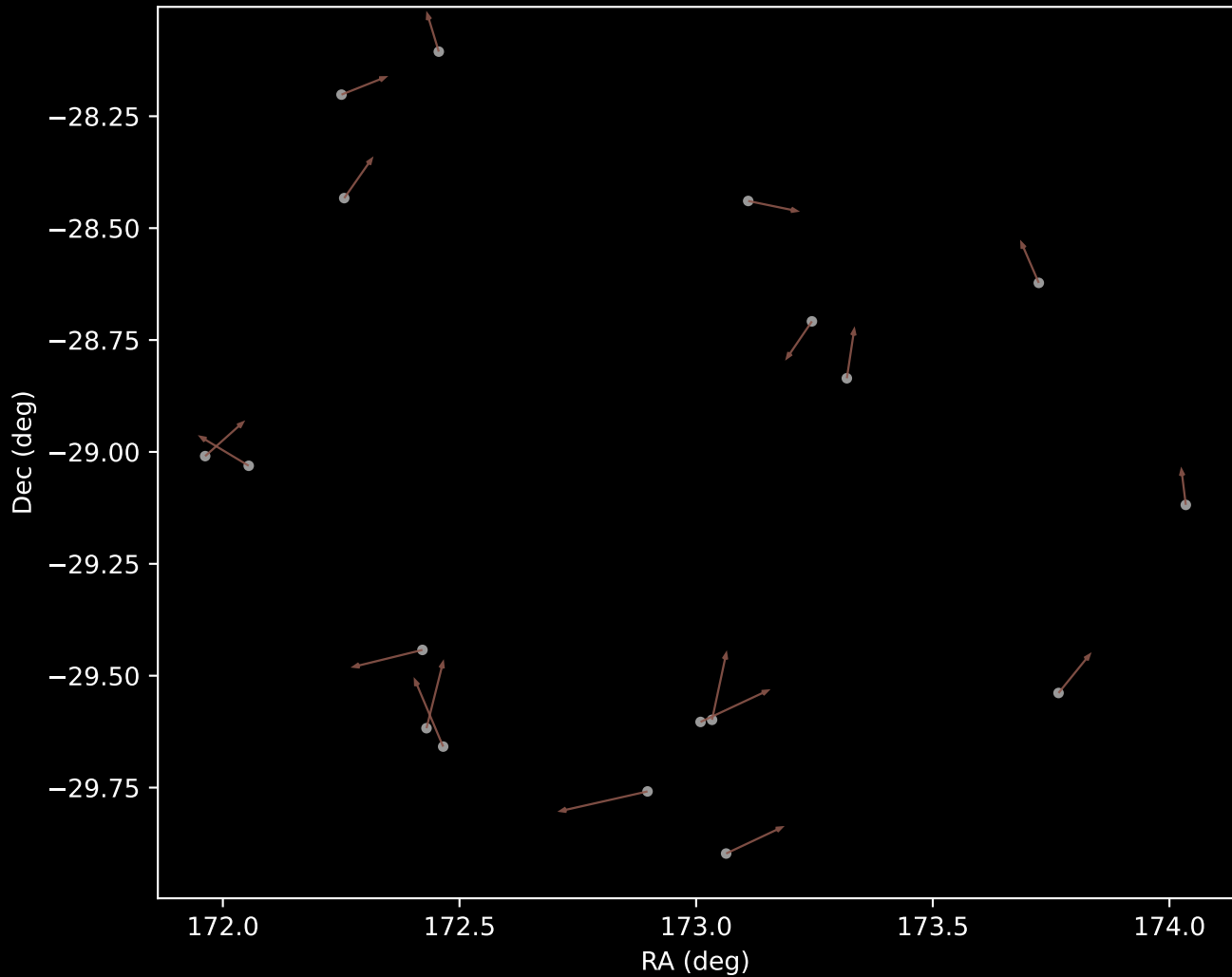
GALAH DR4 Cluster 10 Proper Motion Vectors (n=18)
