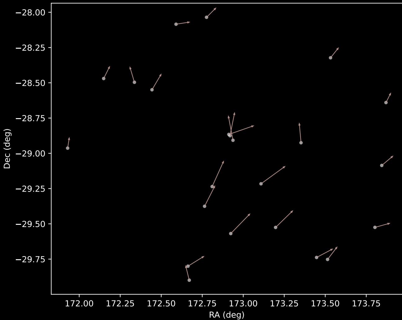
GALAH DR4 Cluster 11 Proper Motion Vectors (n=23)
