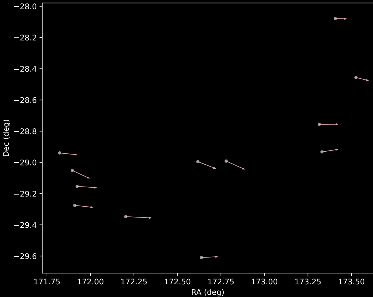
GALAH DR4 Cluster 13 Proper Motion Vectors (n=12)
