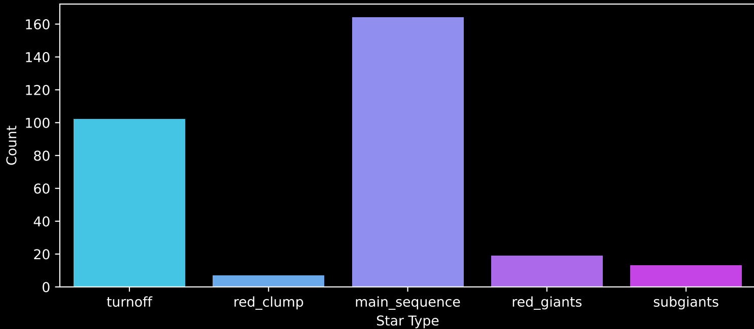
GALAH DR4 Field: [397] Count plot of Star Type
