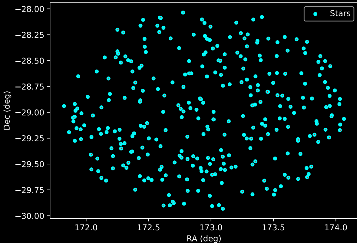
GALAH DR4 Field: [397] Proper Motion Vectors for Gaia Star Field (n= 305)
