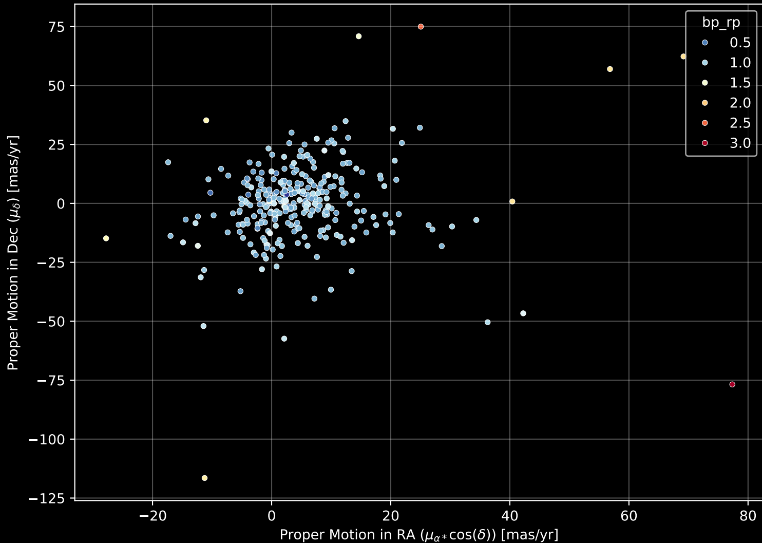
GALAH DR4 Field: [397] Proper Motion Diagram (n= 305)
